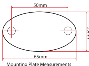
Mounting Plate Measurements
