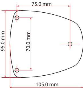
Mounting Plate Measurements
